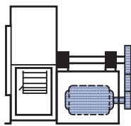
ARR. 9 SWSI. For belt drive. Impeller overhung, two bearings, with prime mover outside base.
