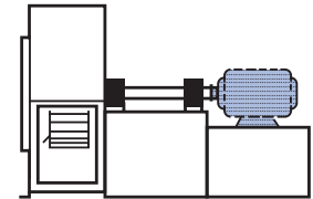
ARR. 8 SWSI. Direct Coupled configuration with motor mounted to common fan base. Impeller is overhung and supported by two bearings on fan base. Temperature Limitations: 250°F.
