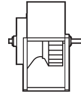
ARR. 3 SWSI. Unit furnished with shaft and bearings, for belt drive configuration. One bearing on each side and supported by fan housing. Temperature limitations: Standard fan to 150° F. (DWDI also available)
