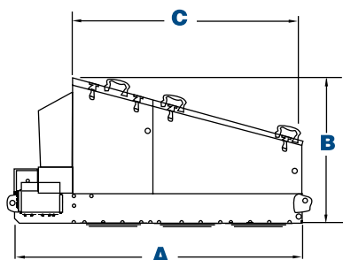
DLMV Type W (Type H plus weather cowl)
