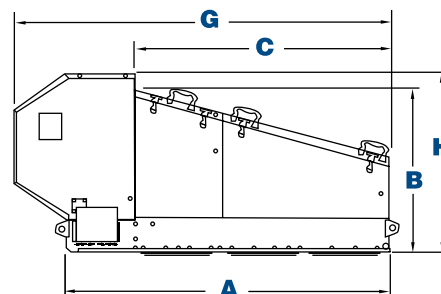
DLMV Type FAD (Type F plus acoustic diffuser)
