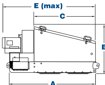
DLMV Type F (Type H plus integral fan)
