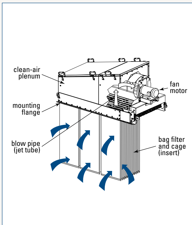
NORMAL OPERATION FOR MODELS DLMV
